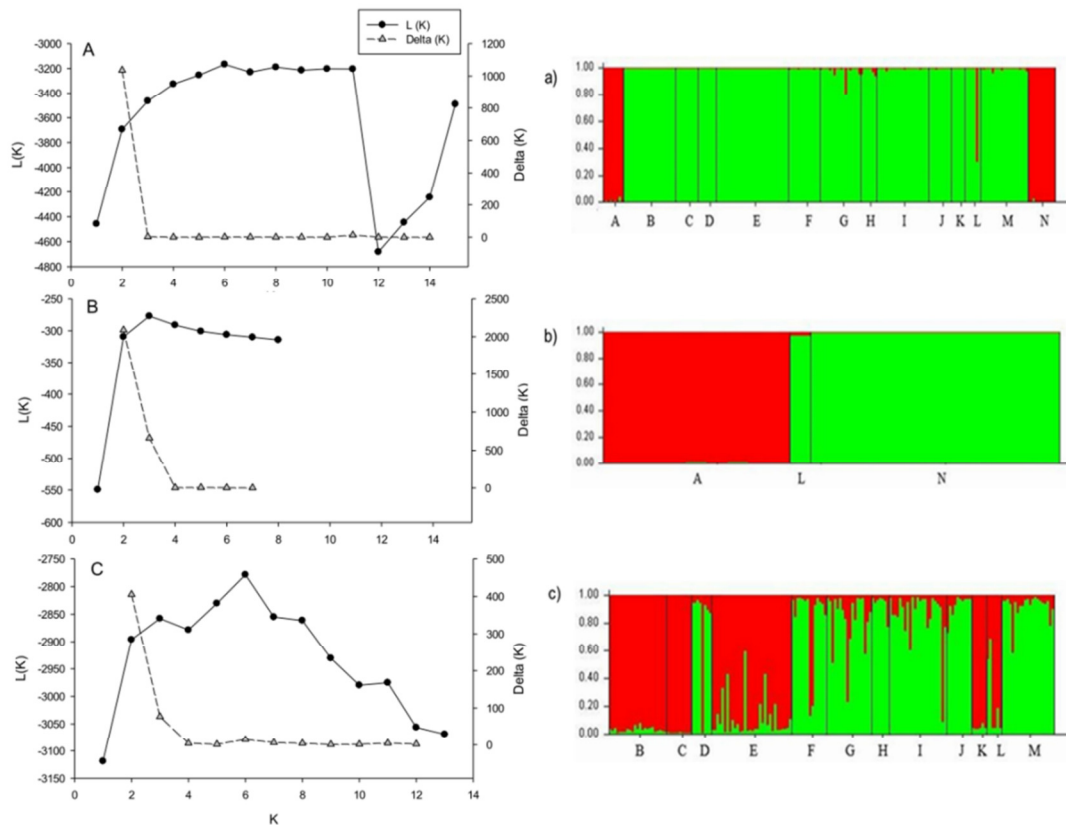
Figure 3: Graphic representation of genetic assignment using STRUCTURE. On the left-hand graph (A, B, C), mean of the natural logarithm of the likelihood L(K) (left y-axis) and of delta K (right y-axis) computed following the Evanno's method (2005) using 10 simulations for each K (x-axis). On the right-hand graphs (a, b, c), the y-axis represent the probability to belong to a certain cluster, while on the x-axes is reported a letter code for each population (see Fig. 1 and Tab. 1). Each colour represents a cluster and each vertical bar a single
