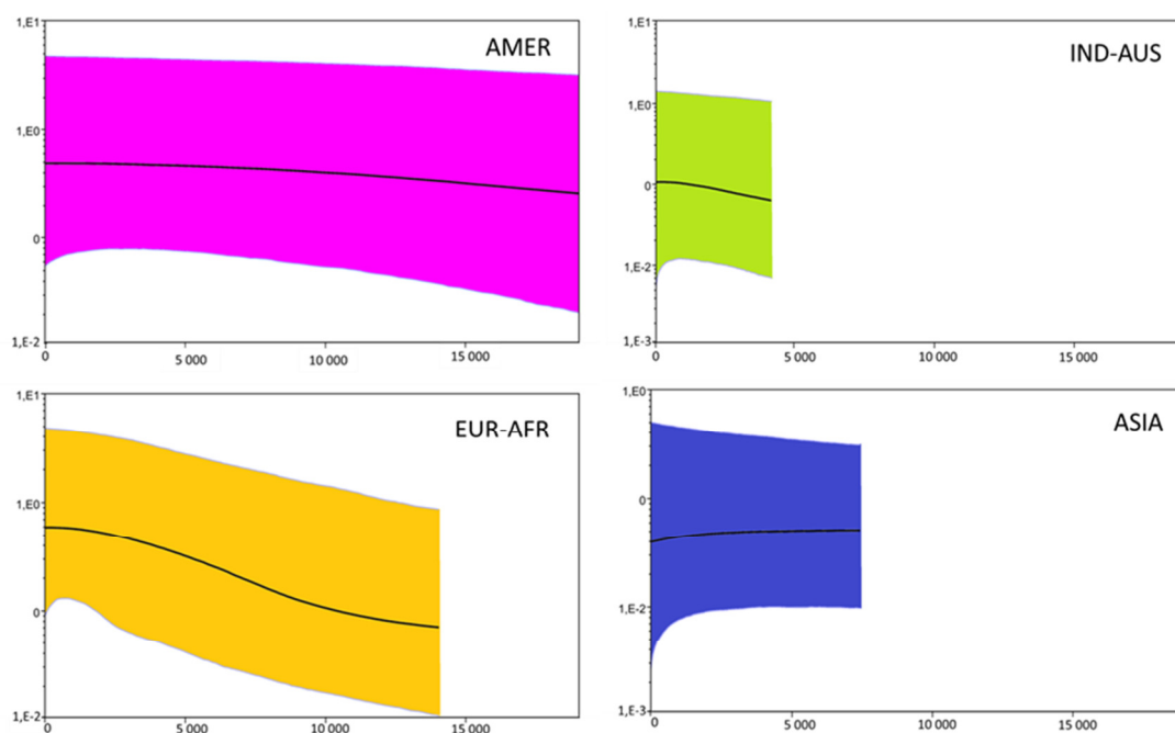
Figure 4: Bayesian skyline plots showing the demographic histories of the four main haplogroups identified in the Pandion haliaetus sequences. On the x-axis the time is
