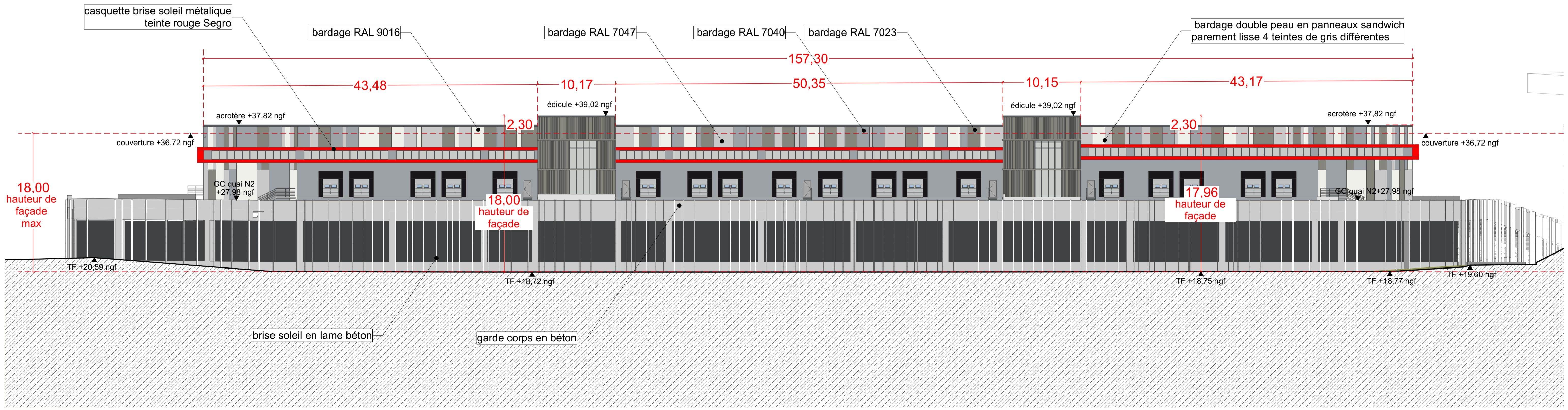
Facade Sud - 1/250
