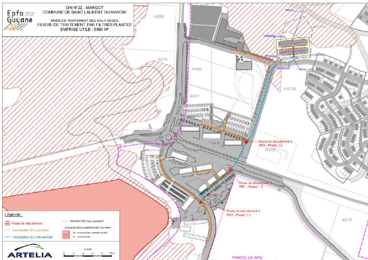
Figure 5 - Extrait annexe B plan masse EU solution retenue
